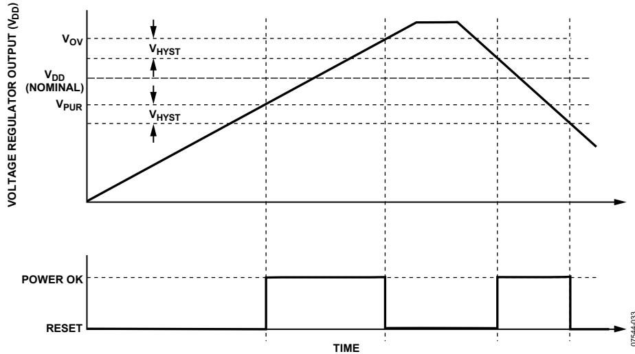
Figure 33. Voltage Regulator Monitor Reset Functionality
